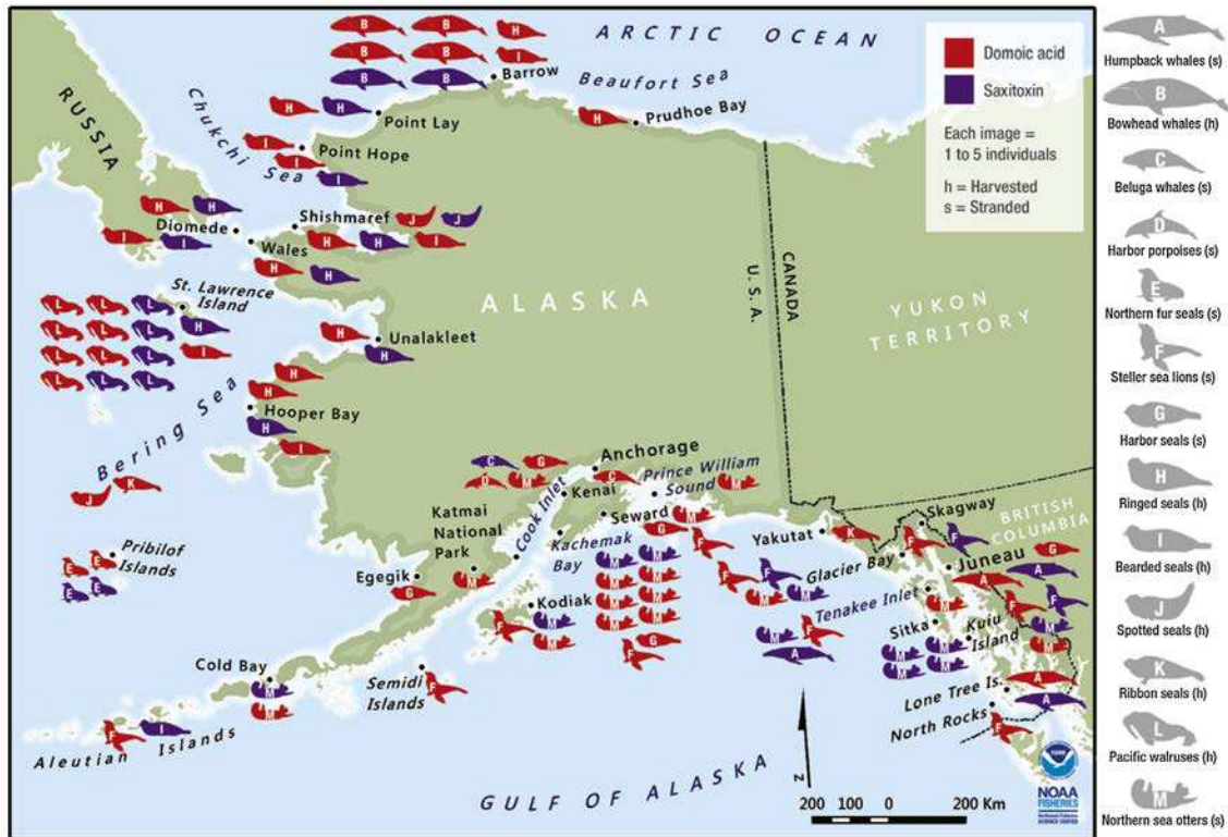
Figure 23. Algal toxins detected in 13 species of marine mammals from southeast Alaska to the Arctic from 2004 to 2013 (Lefebvre et al. 2016).
