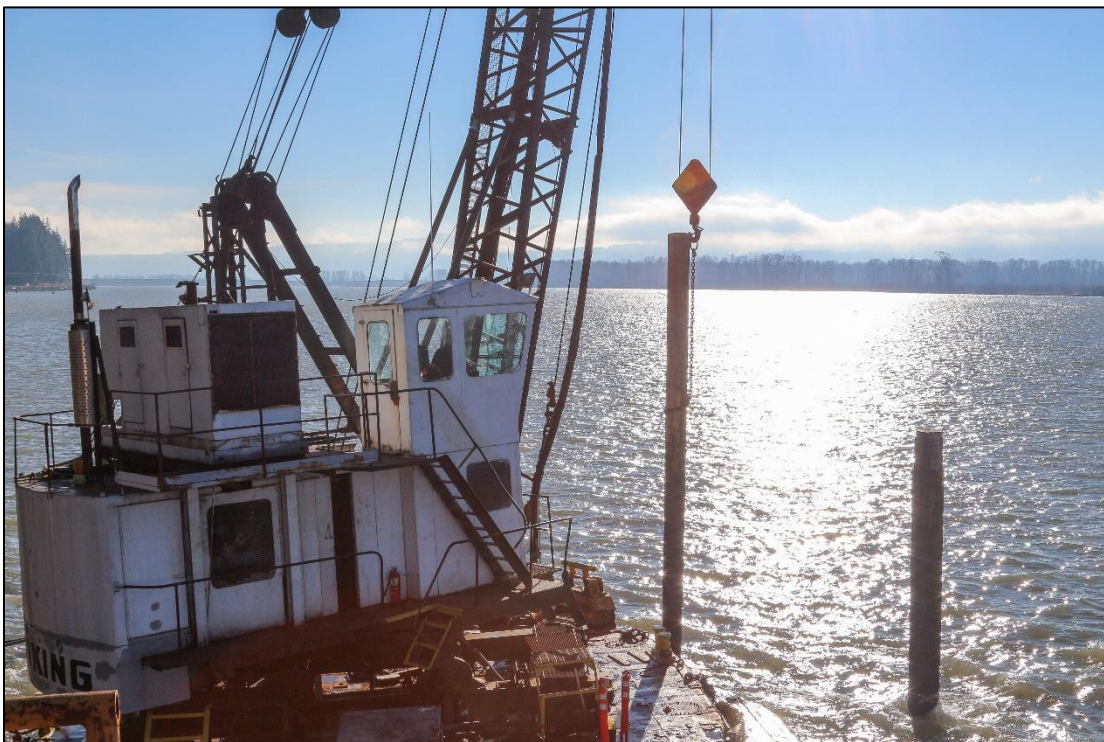
Figure D-2. WFC designing the trap configuration and piling layout based upon historical research.
